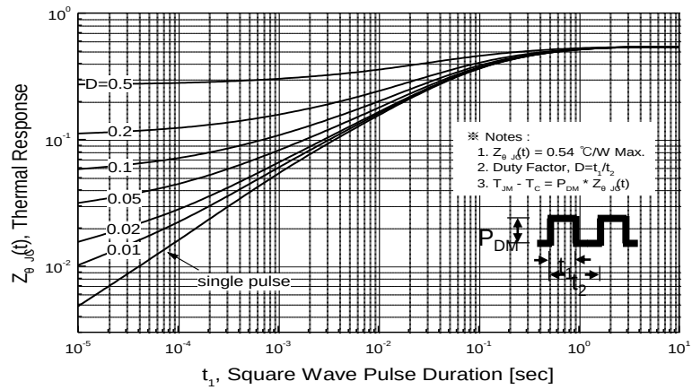
Figure 12. Transient Thermal Response Curve for PFP12N65
