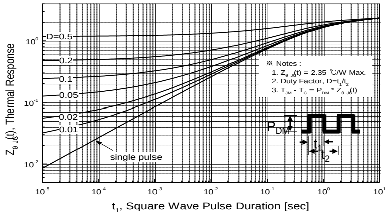
Figure 13. Transient Thermal Response Curve for PFF12N65
