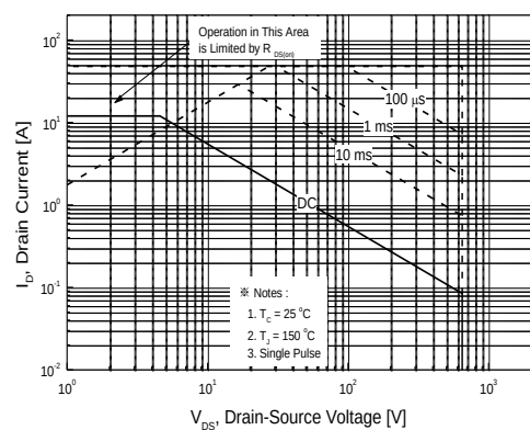
Figure 10. Maximum Safe Operating Area for PFF12N65
