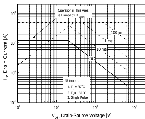
Figure 9. Maximum Safe Operating Area for PFP12N65
