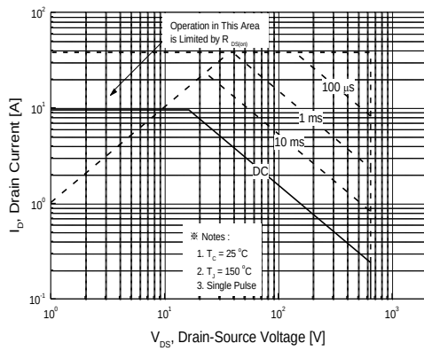
Figure 9. Maximum Safe Operating Area for PFP10N65
