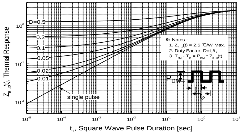
Figure 13. Transient Thermal Response Curve for PFF10N65
