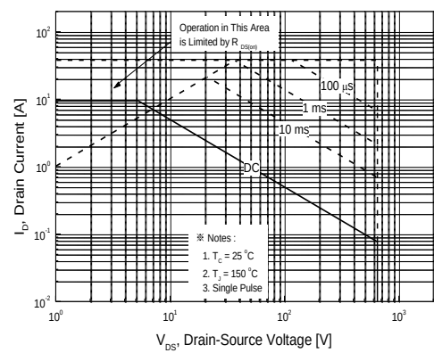
Figure 10. Maximum Safe Operating Area for PFF10N65
