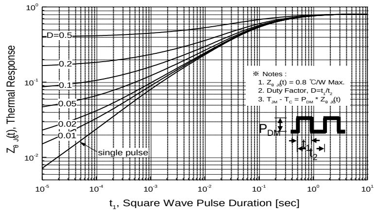
Figure 12. Transient Thermal Response Curve for PFP10N65
