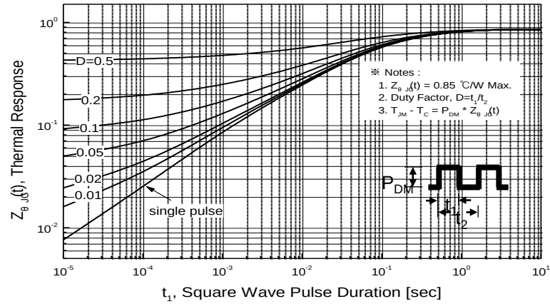
Figure 12. Transient Thermal Response Curve for PFP7N65E
