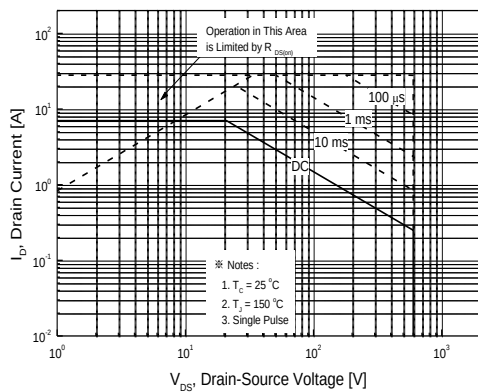
Figure 9.1 Maximum Safe Operating Area for PFP7N65E
