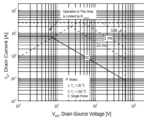
Figure 9.2 Maximum Safe Operating Area for PFF7N65E
