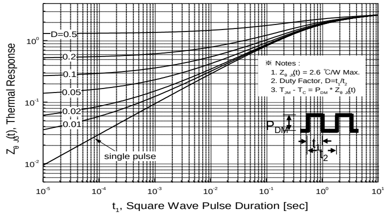
Figure 13. Transient Thermal Response Curve for PFF7N65E
