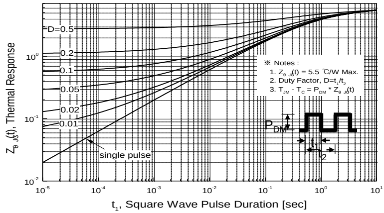
Figure 13. Transient Thermal Response Curve for PFF2N65
