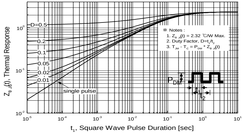
Figure 12. Transient Thermal Response Curve for PFP2N65
