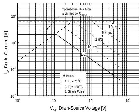
Figure 10. Maximum Safe Operating Area for PFF2N65
