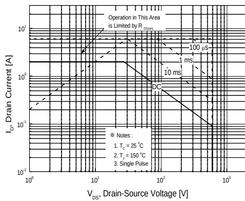
Figure 9. Maximum Safe Operating Area for PFP2N65
