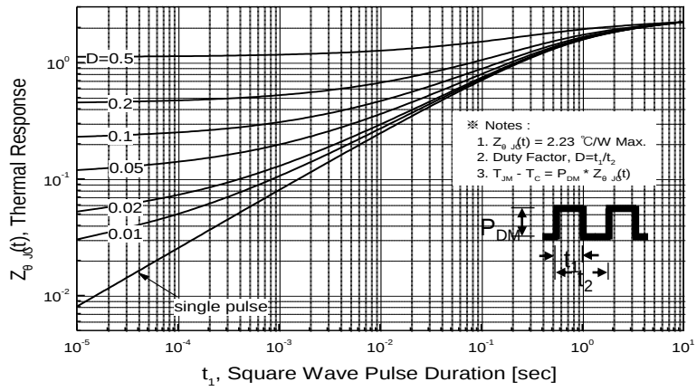
Figure 13. Transient Thermal Response Curve for PFF13N50
