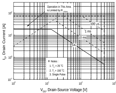
Figure 9. Maximum Safe Operating Area for PFP18N50
