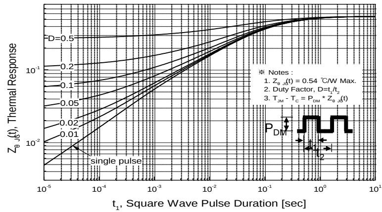
Figure 12. Transient Thermal Response Curve for PFP18N50
