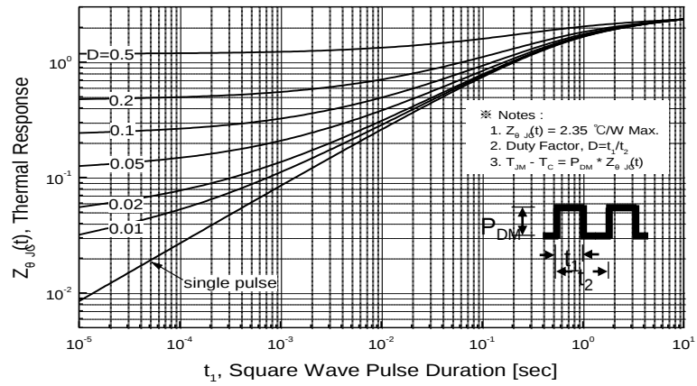
Figure 13. Transient Thermal Response Curve for PFF18N50
