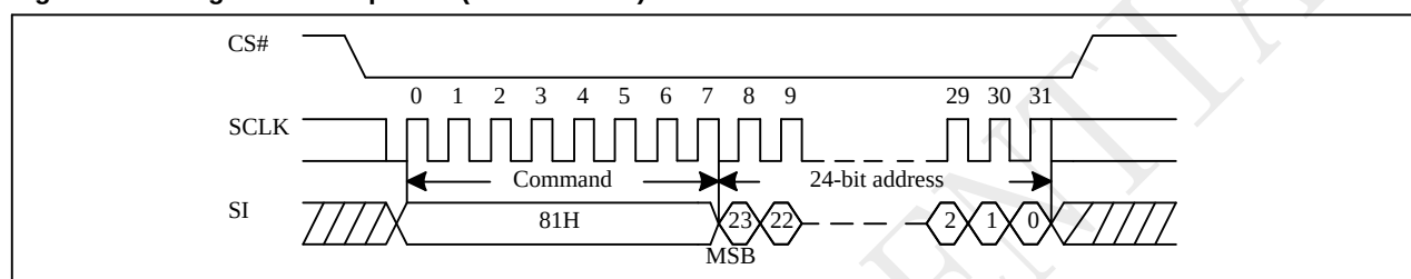
Figure 10-17 Page Erase Sequence (Command 81)
