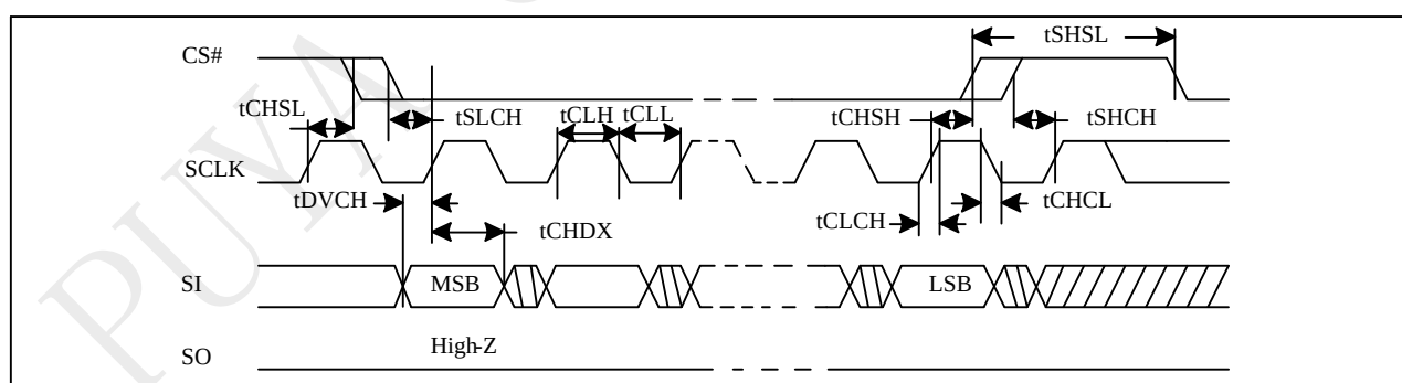
Figure 5-4 Serial Input Timing
