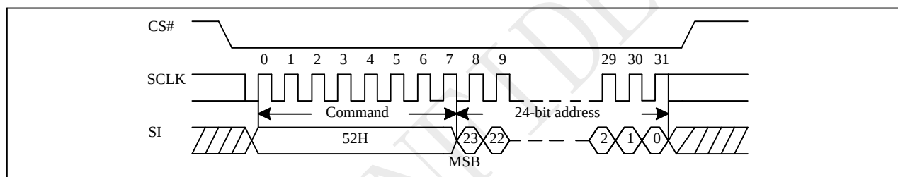
Figure 10-19 Block Erase 32K(BE32K) Sequence (Command 52)
