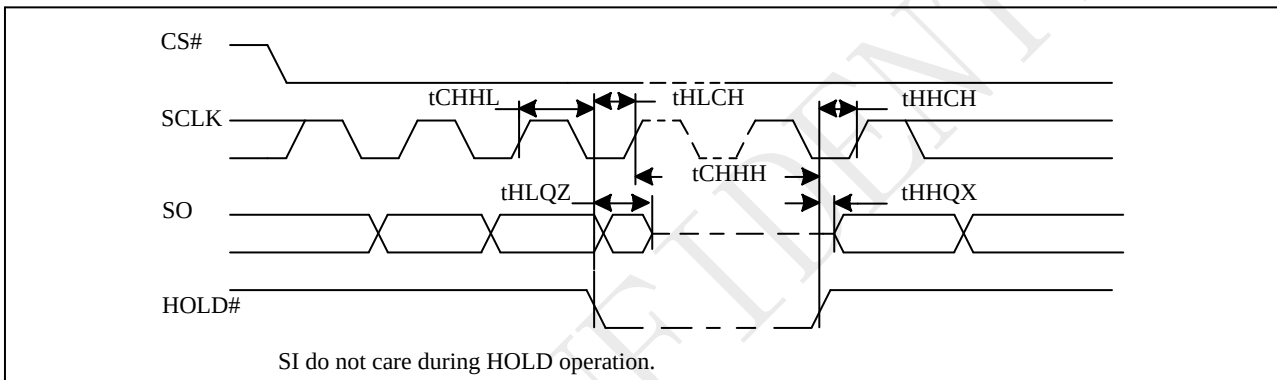
Figure 5-6 Hold Timing
