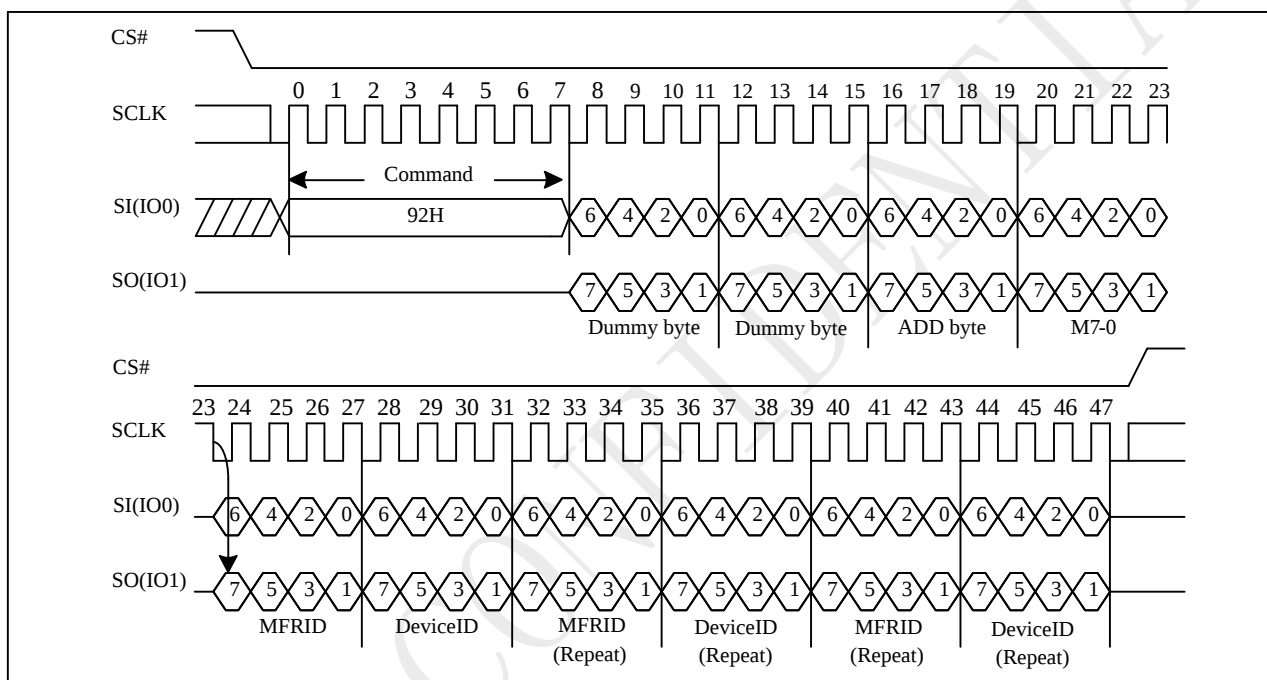
Figure 10-31 DUAL I/O Read Electronic Manufacturer & Device ID (DREMS) Sequence (Command 92)
