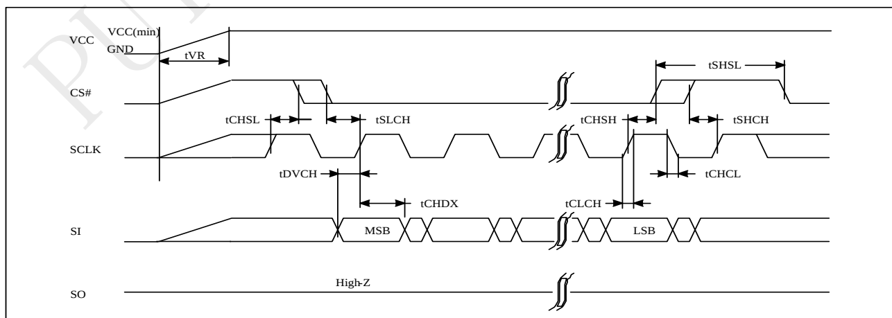
Figure 5-8 AC Timing at Device Power-Up
