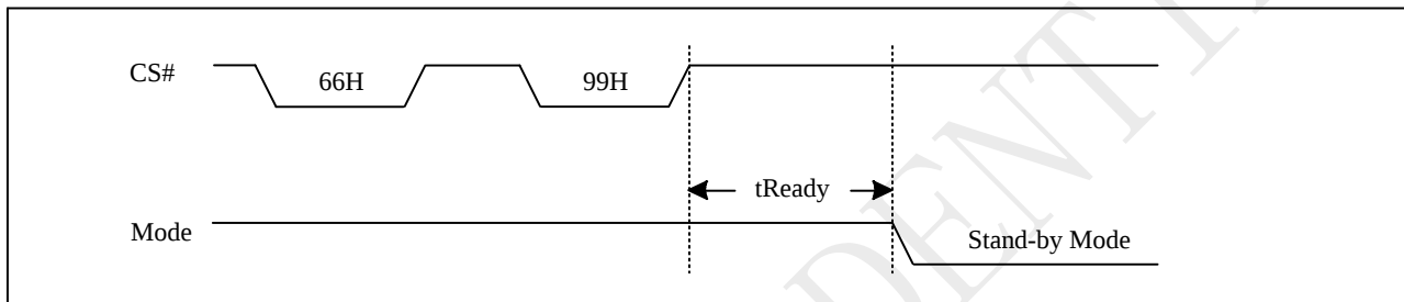
Figure 10-41 Reset Sequence
