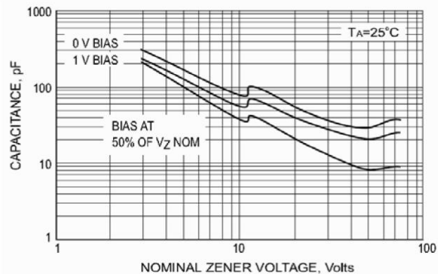
Fig.4 TYPICAL CAPACITANCE
