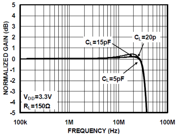
Figure 3 Gain Vs. Frequency with C_{LOAD} (HD Channel)
