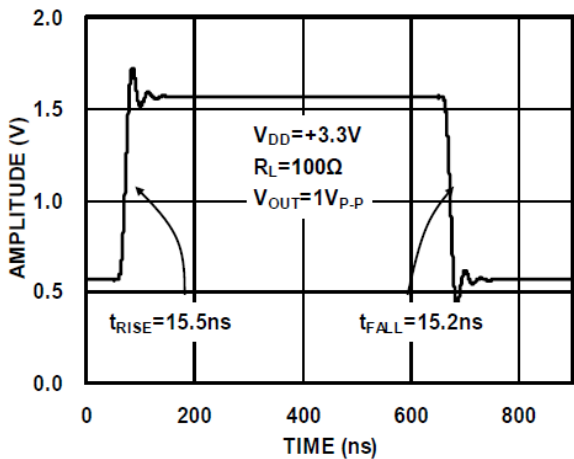
Figure 9 Large-Signal Pulse Response Vs. Time (HD Channel)
