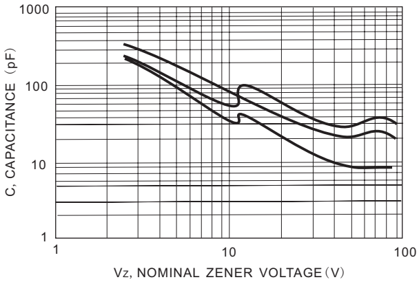
Figure 7. Typical Capacitance
