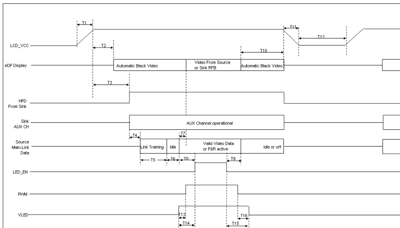
Figure 12 Power Sequence
