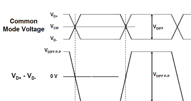
Figure 8 Display Port Main Link Signal
