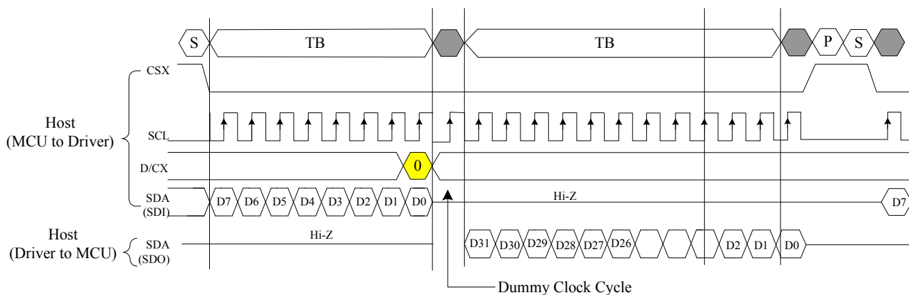
Figure8: 4-pins Serial Protocol (for 09H command: 32-bit read)
