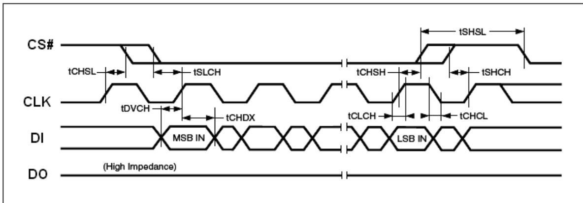
Input Timing
