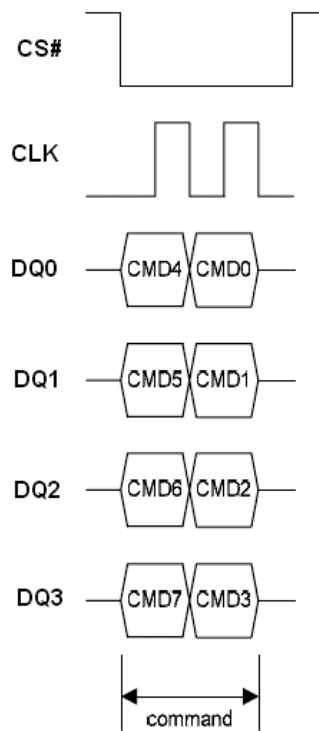
Chip Erase Sequence in QPI Mode
