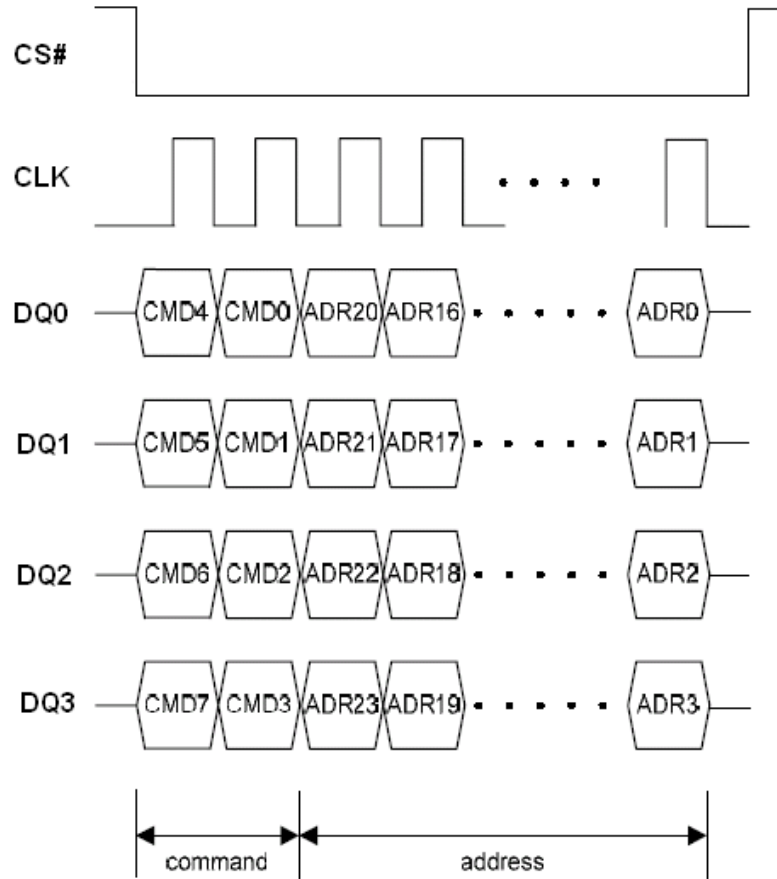
Half Block/Block/Sector Erase Instruction Sequence in QPI Mode
