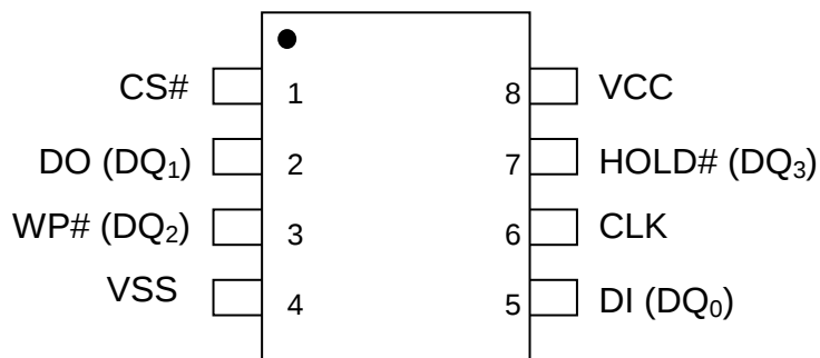
8 - LEAD SOP / PDIP
