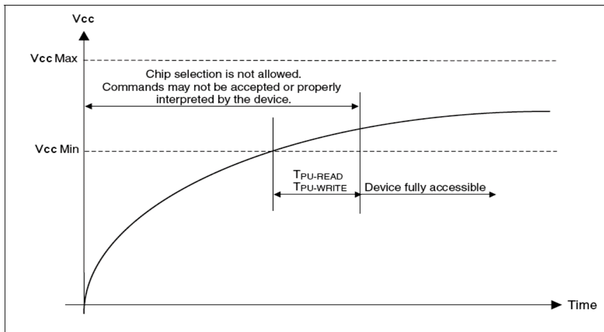
Power-up Timing
