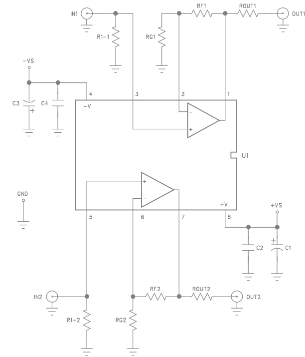
Figure 9. CEB006 Schematic
