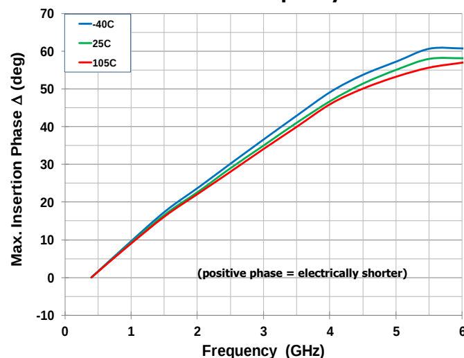
Max. Insertion Phase \Delta vs. Frequency
