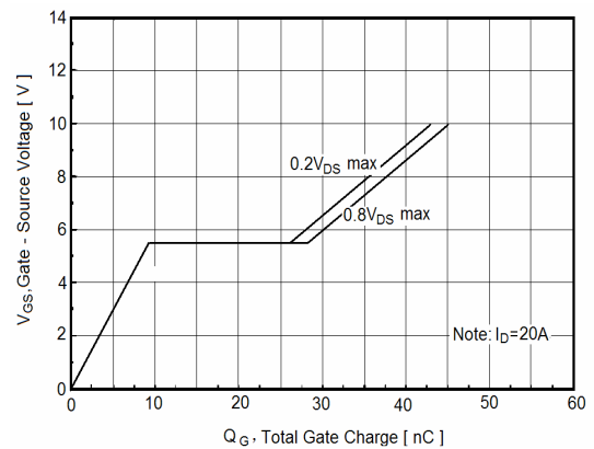
Figure 10. Gate Charge Waveforms
