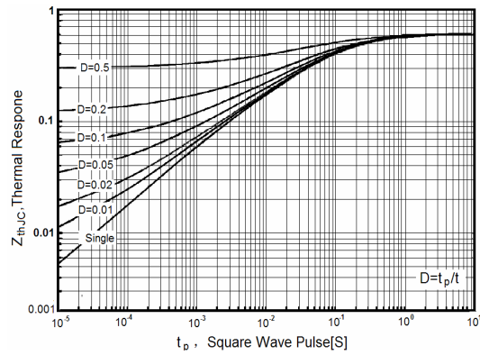
Figure 12. Transient Thermal Response Curve (TO-220)
