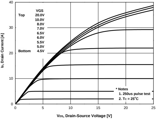
Output Characteristics
