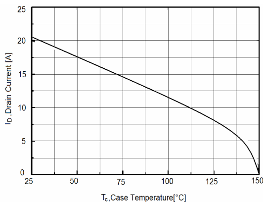
Figure 9. Maximum I_D vs. Junction Temperature
