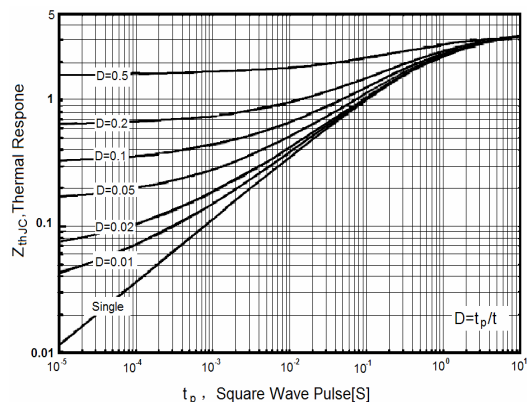
Figure 13. Transient Thermal Response Curve (TO-220F)
