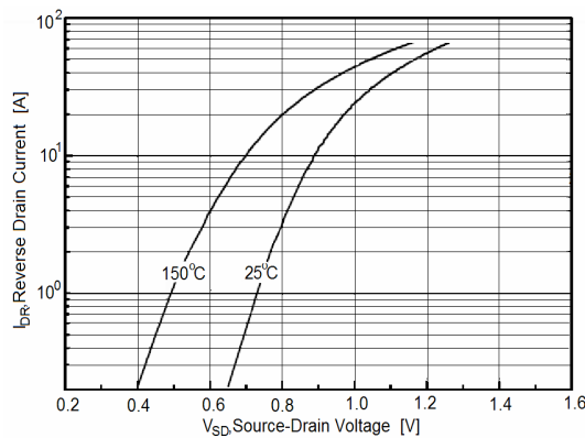
Figure 3. Source-Drain Diode Forward Voltage
