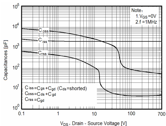
Figure 11. Capacitance
