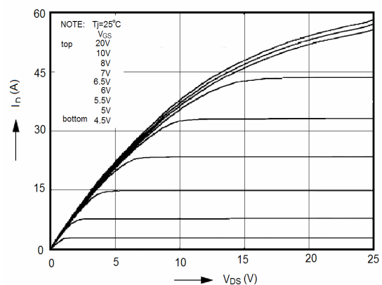
Figure 4. Output Characteristics
