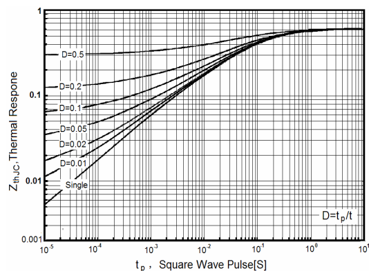
Figure 12. Transient Thermal Response Curve (TO-220)
