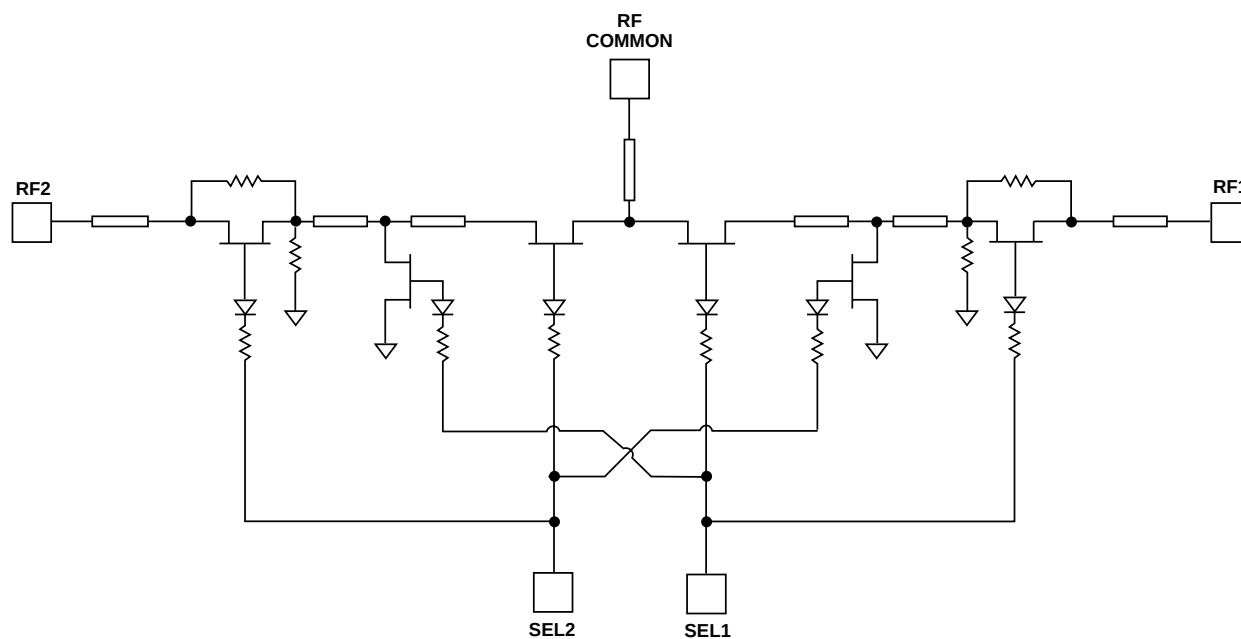
Figure 1. HMMC-2007 Schematic.
