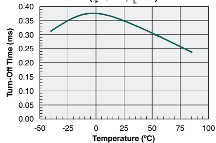
Typical Turn-Off Time vs. Temperature ( I_F=5\text{mA} , I_L=1\text{A} )
