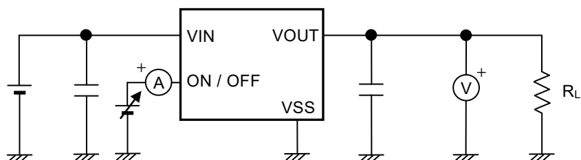
Figure 9 Test Circuit 3
