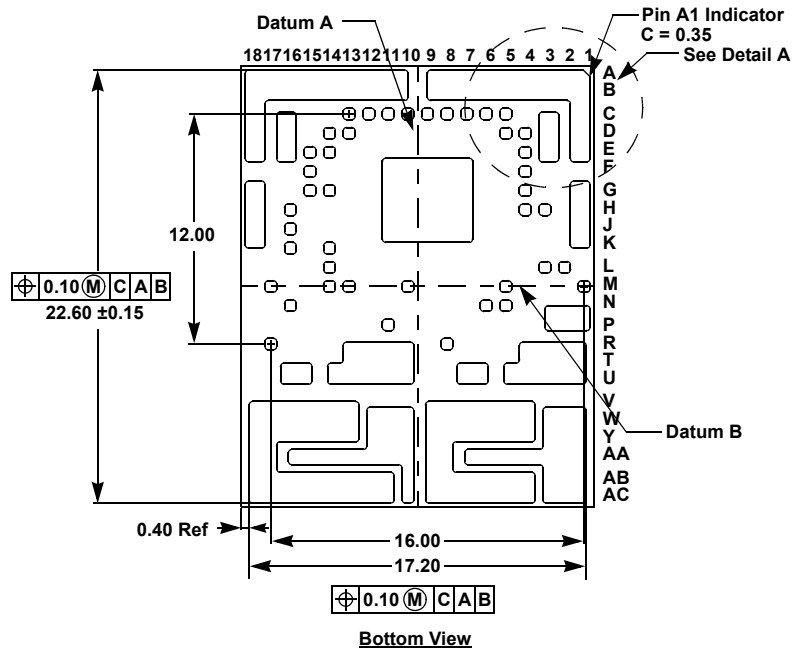
Bottom View
