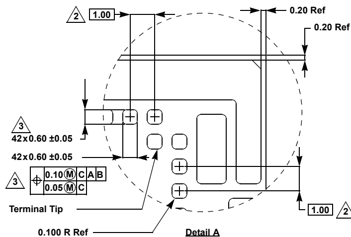
Detail A
