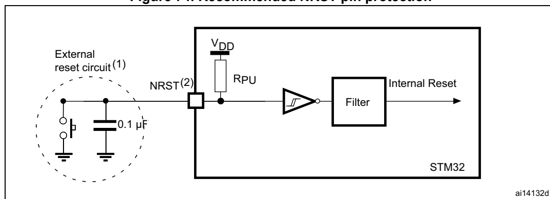
Figure 74. Recommended NRST pin protection
