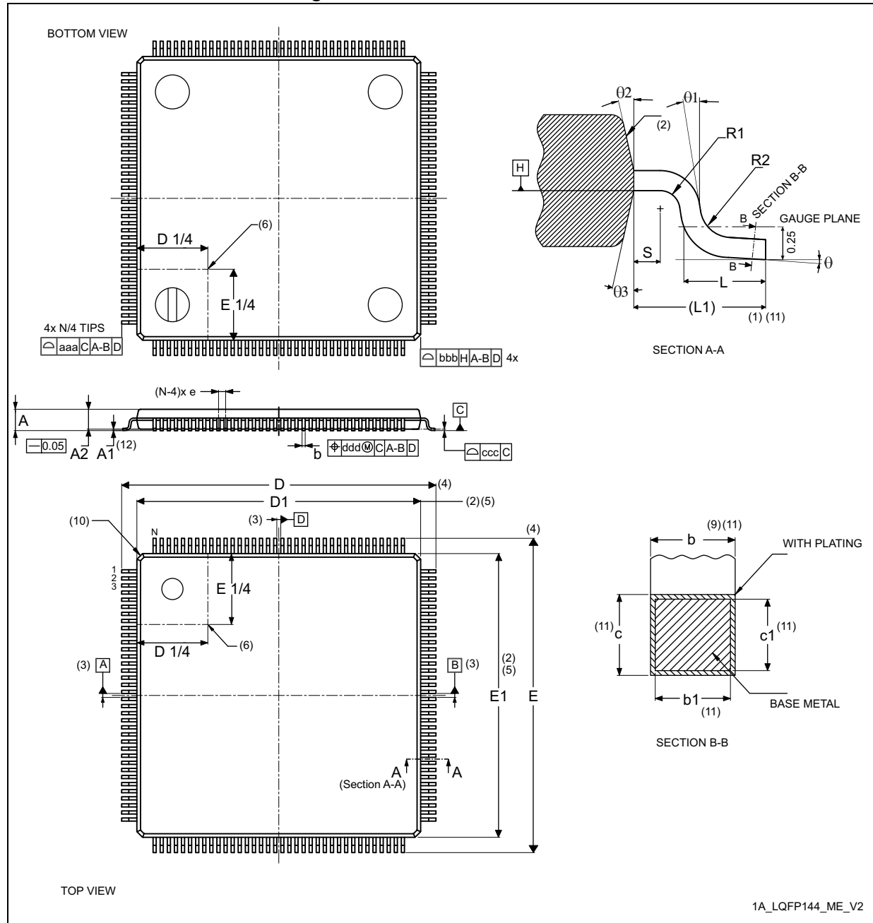
Figure 120. LQFP144 - Outline (15)
