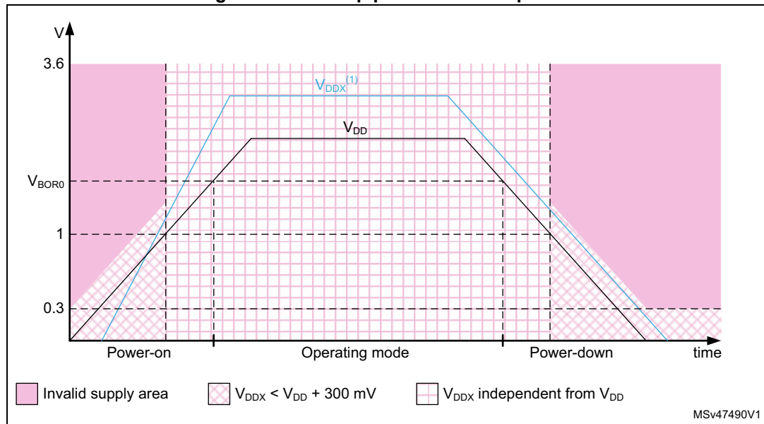
Figure 3. Power-up/power-down sequence
