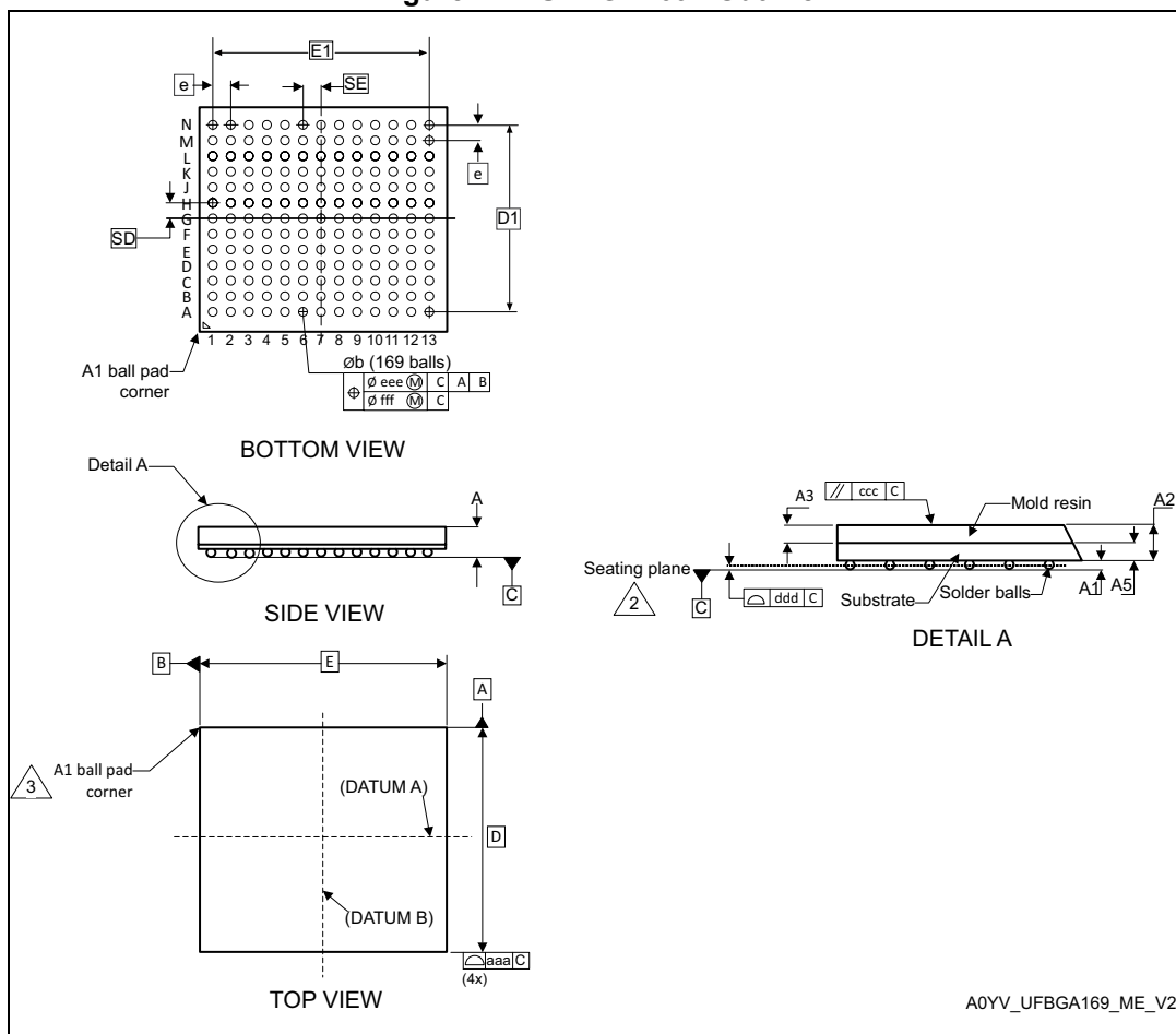
Figure 122. UFBGA169 - Outline
