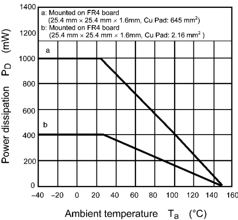
Fig. 8.13 P_D - T_a
