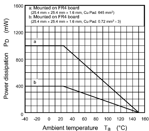
Fig. 7.12 P_D - T_a
