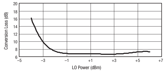
Figure 9. Conversion Loss vs LO Power
