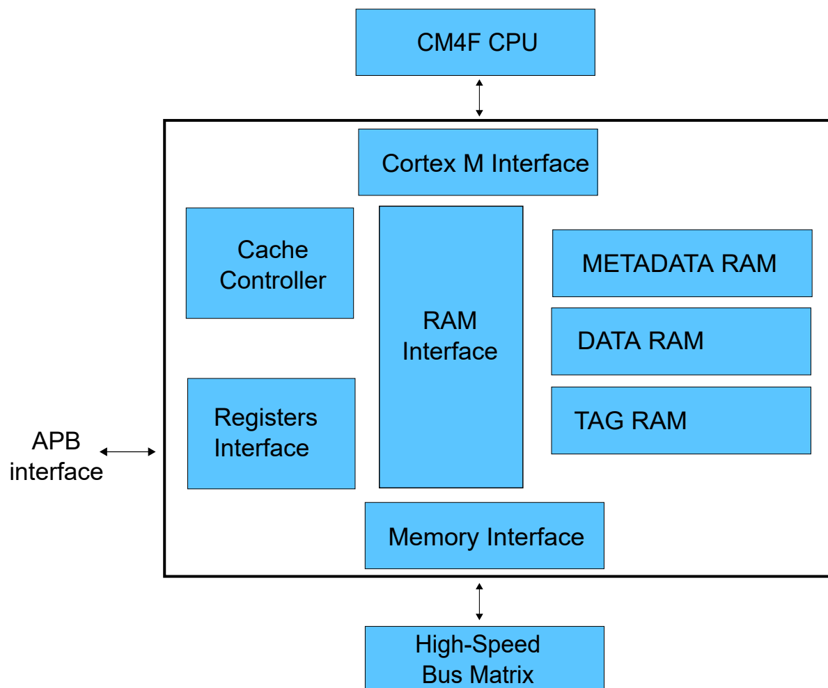
Figure 11-1. CMCC Block Diagram
