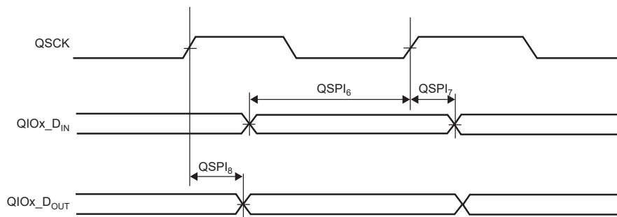
Figure 54-13. QSPI SDR Host Mode 3
