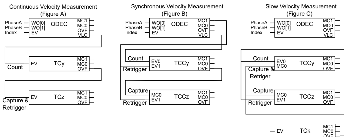
Figure 53-9. Speed Measurement
