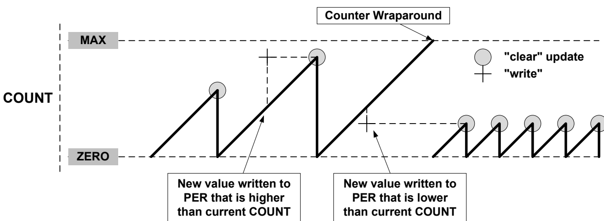
Figure 49-10. Unbuffered Single-Slope Up-Counting Operation
