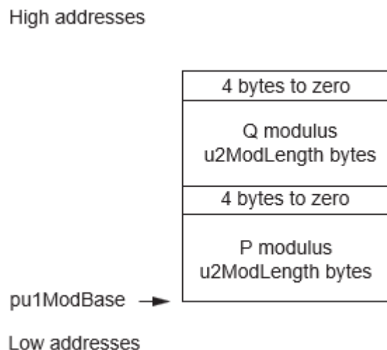
Figure 43-2. Modulus P and Q in {nu1ModBase, 2*u2ModLength + 8}
