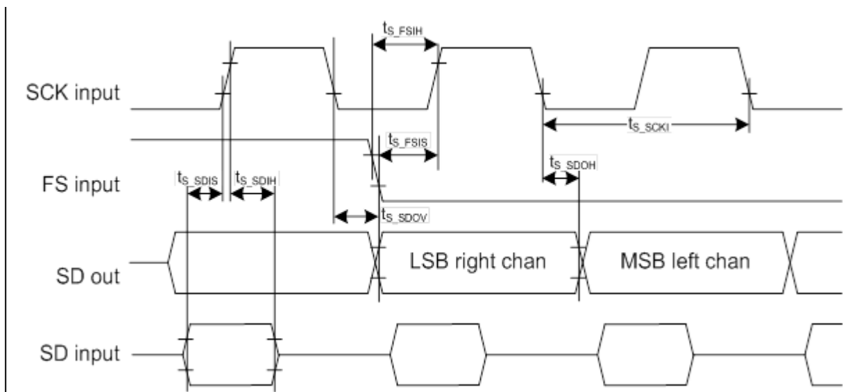
Figure 54-20. Client Mode: SCK and FS are Input
