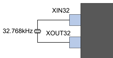
Figure 60-10. External Real Time Oscillator without Load Capacitor
