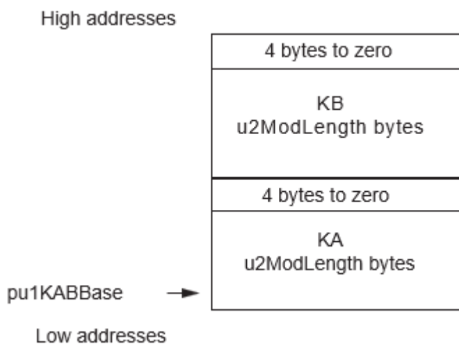
Figure 43-9. Scalars KA and KB {pu1KABBase, 2 * u2KLength + 8}
