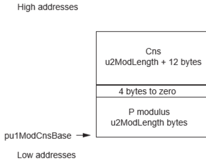
Figure 43-7. Modulus P and Cns{pu1ModCnsBase, 2 * u2ModLength + 16 }
