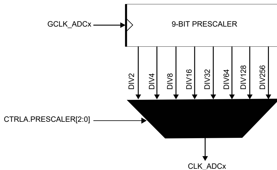
Figure 45-2. ADC Prescaler
