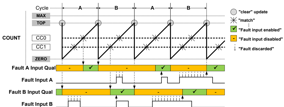
Figure 49-24. Fault Qualification in RAMP2 Operation with Inverted Polarity
