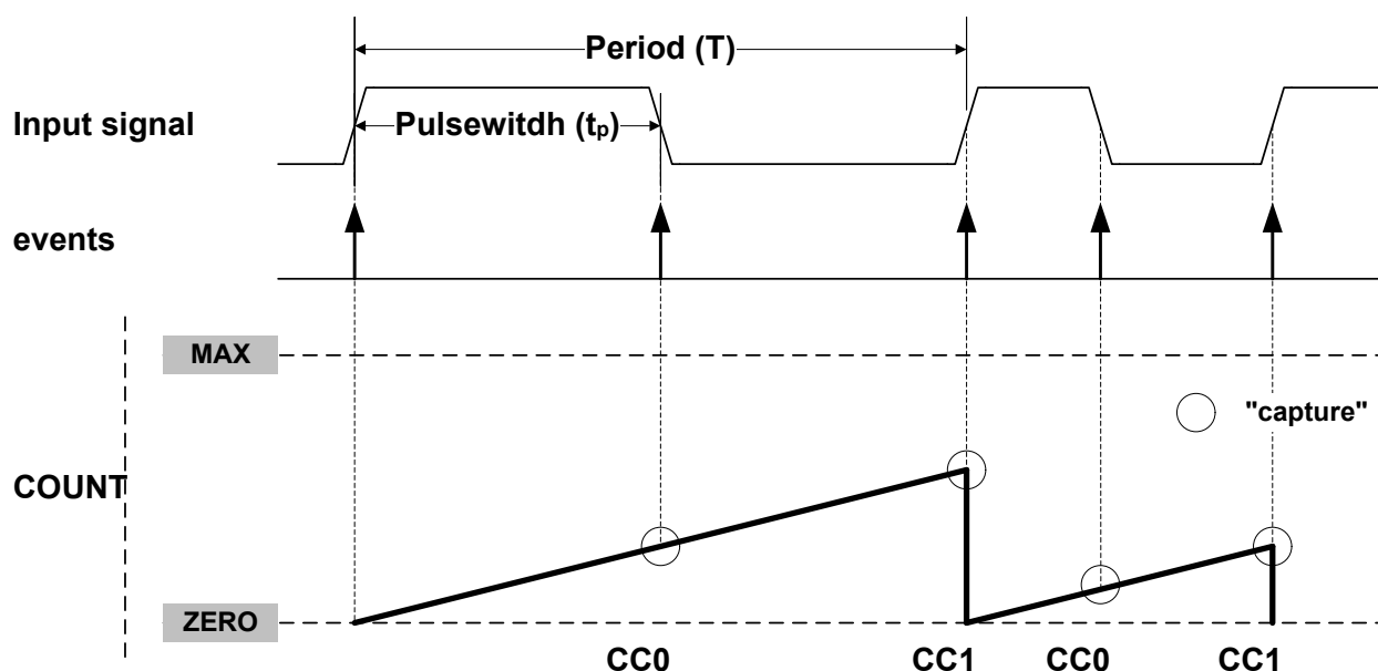
Figure 48-13. PWP Capture
