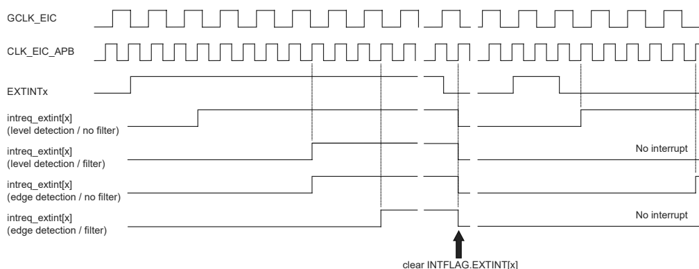
Figure 23-2. Interrupt Detection Latency by modes (Rising Edge)
