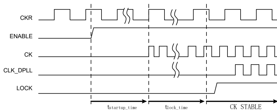
Figure 28-4. CK and CLK_DPLL Output from DPLL Off Mode to Running Mode
