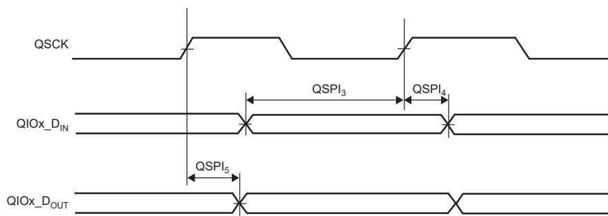
Figure 54-11. QSPI SDR Host Mode 1
