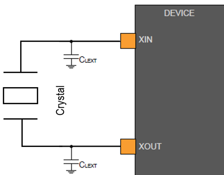
Figure 54-5. Oscillator Connection
