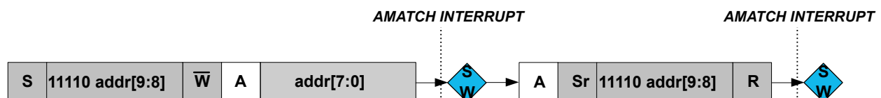
Figure 36-11. 10-bit Addressing
