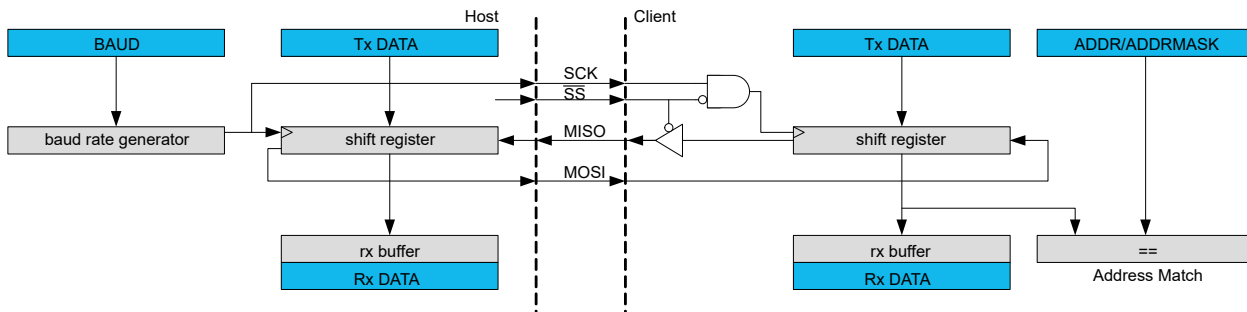
Figure 35-1. Full-Duplex SPI Host Client Interconnection
