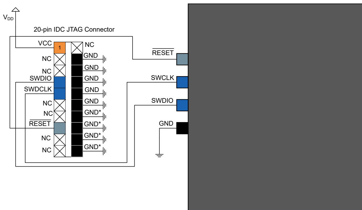
Figure 60-15. 20-pin IDC JTAG Connector
