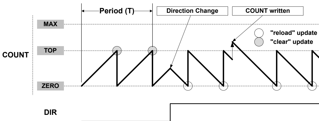
Figure 48-3. Counter Operation
