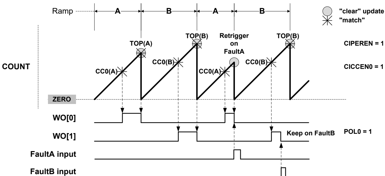
Figure 49-19. RAMP2 Alternate Operation
