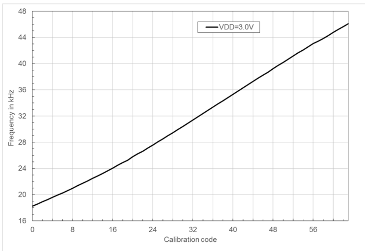
Figure 54-7. Average Frequency Versus Calibration Code Value, VDD = 3V
