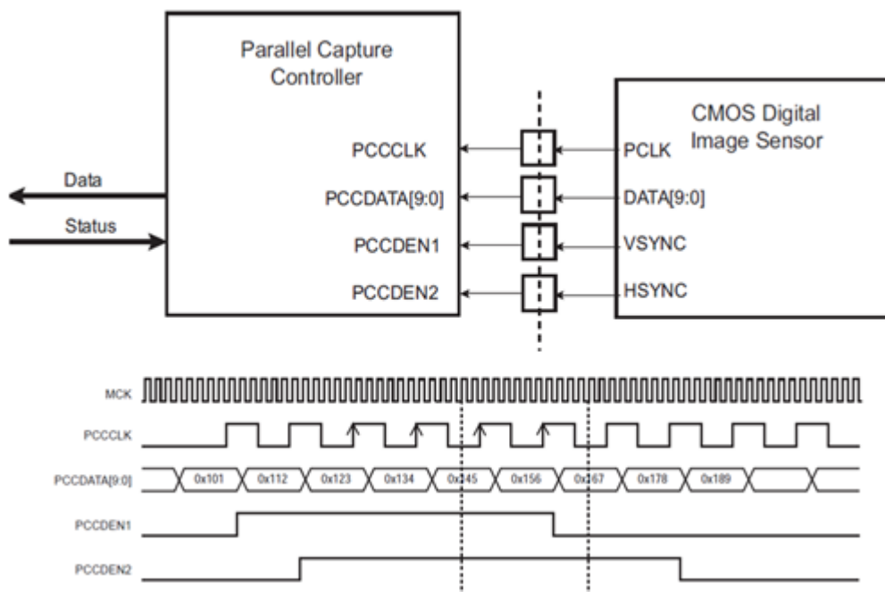
Figure 54-22. PCC Signaling
