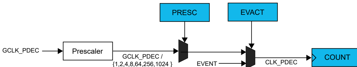
Figure 53-2. Prescaler Selection
