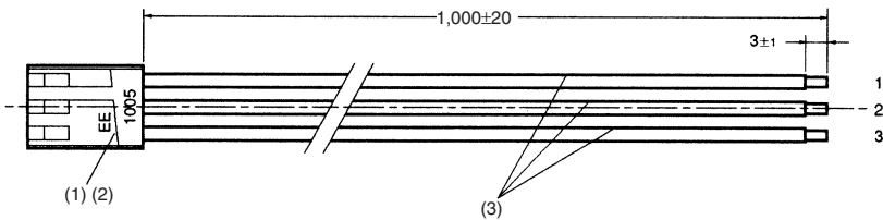
EE-1005 Connector
