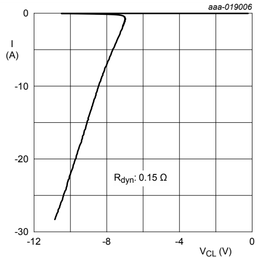
Fig. 6. Dynamic resistance
