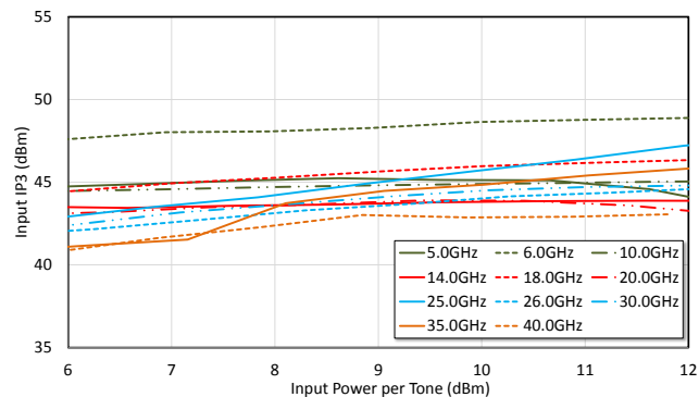
Input IP3 vs. SCL Input Power @ V_{C1} = -2.0 V, V_{C2} = -2.0 V
