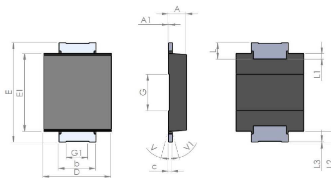
Figure 12. SMB Flat package outline
