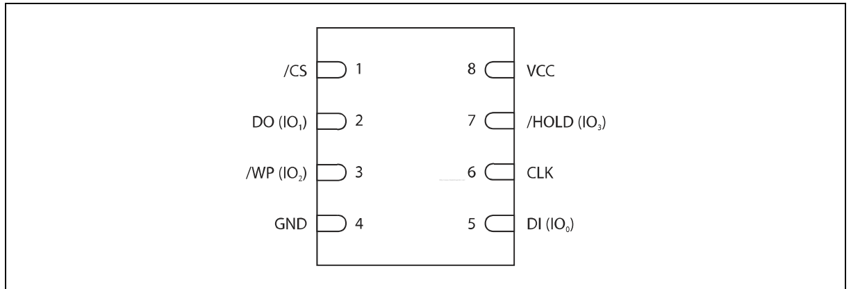
Figure 1b. W25Q80, W25Q16 Pad Assignments, 8-pad WSON (Package Code ZP)
