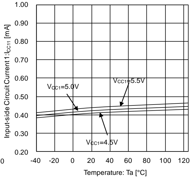
Figure 8. Input-side Circuit Current 1 vs Temperature
