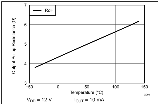
Figure 9. Output Pullup Resistance vs Temperature
