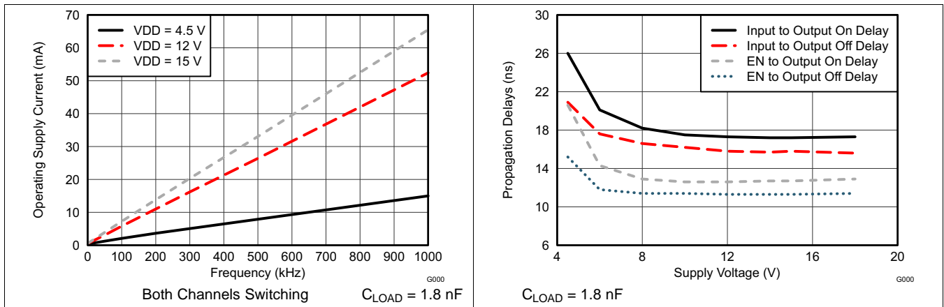
Figure 15. Operating Supply Current vs Frequency
