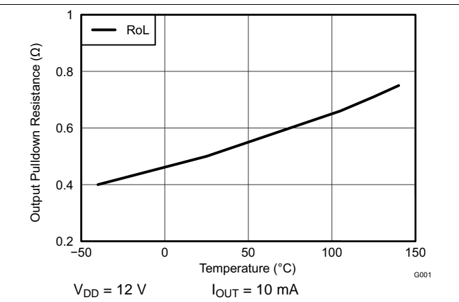
Figure 10. Output Pulldown Resistance vs Temperature
