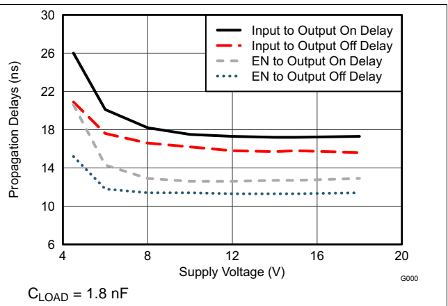
Figure 16. Propagation Delays vs Supply Voltage
