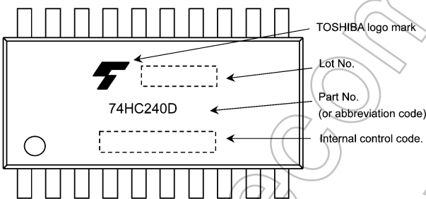
74HC240D
