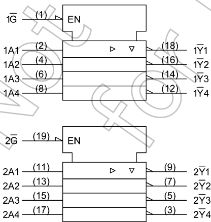
74HC240D
