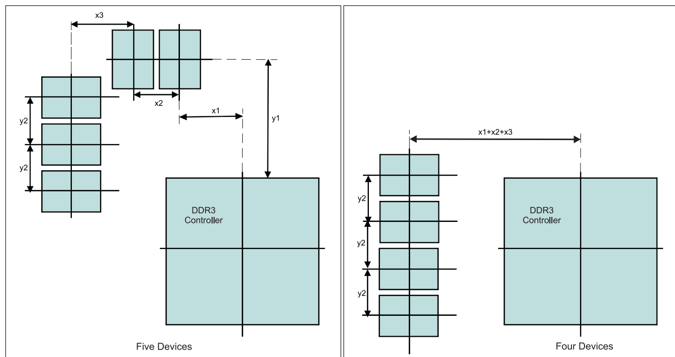
Figure 7-40. Placement Specifications
