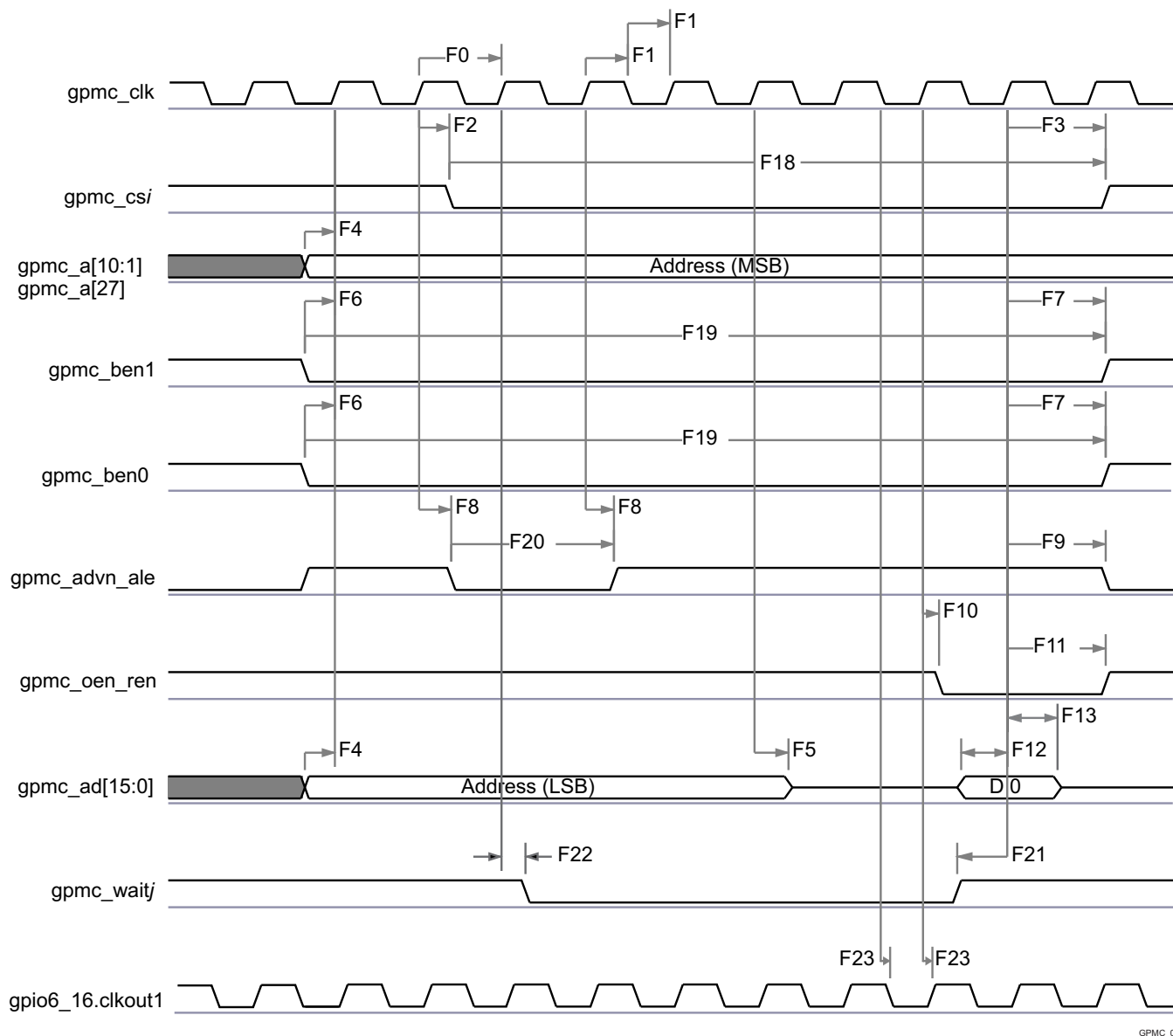
Figure 5-23. GPMC / Multiplexed 16bits NOR Flash - Synchronous Single Read - (GpmcFCLKDivider = 0) (1)(2)
