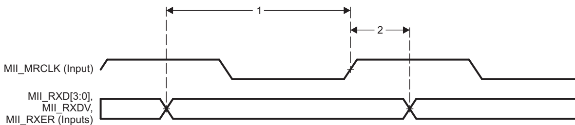
Figure 5-127. PRU-ICSS MII_RXD[3:0], MII_RXDV, and MII_RXER Timing
