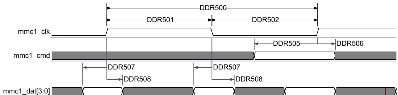
Figure 5-90. SDMMC - High Speed SD - DDR - Data/Command Receive
