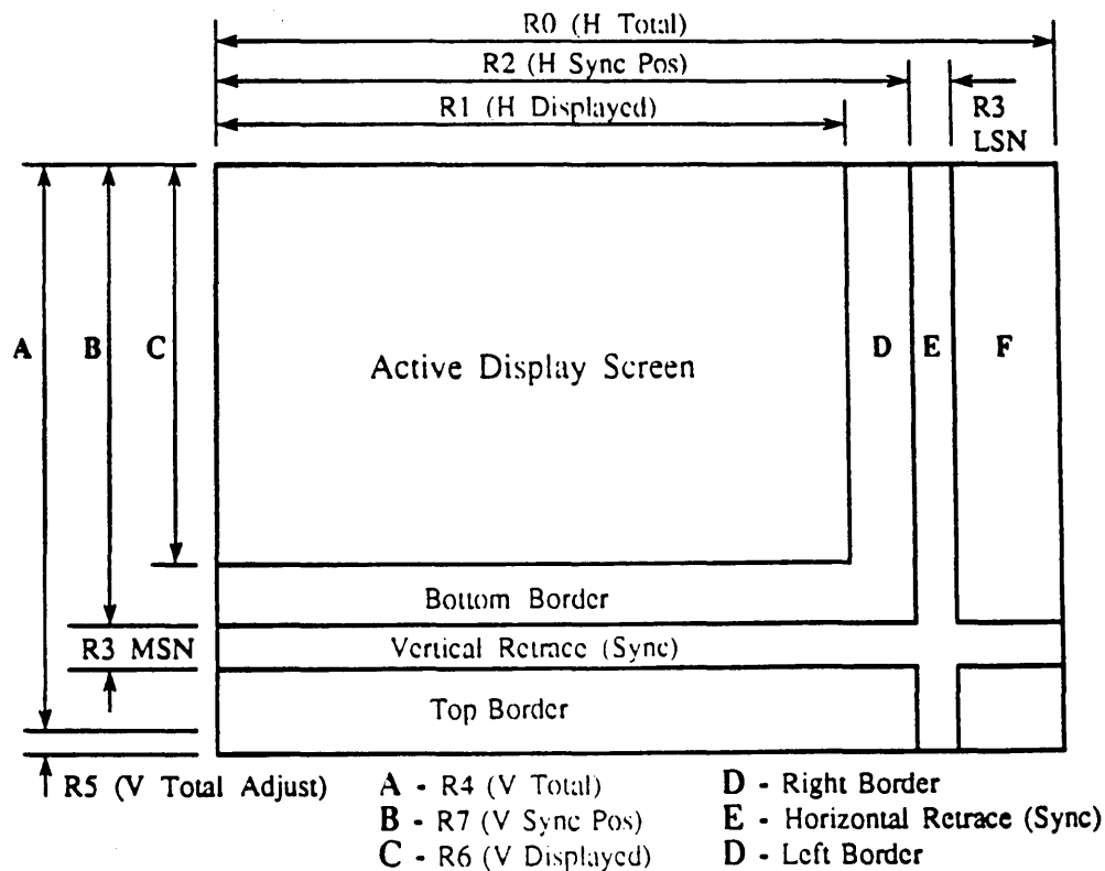
Figure 4-1: 6845 Timing Registers
