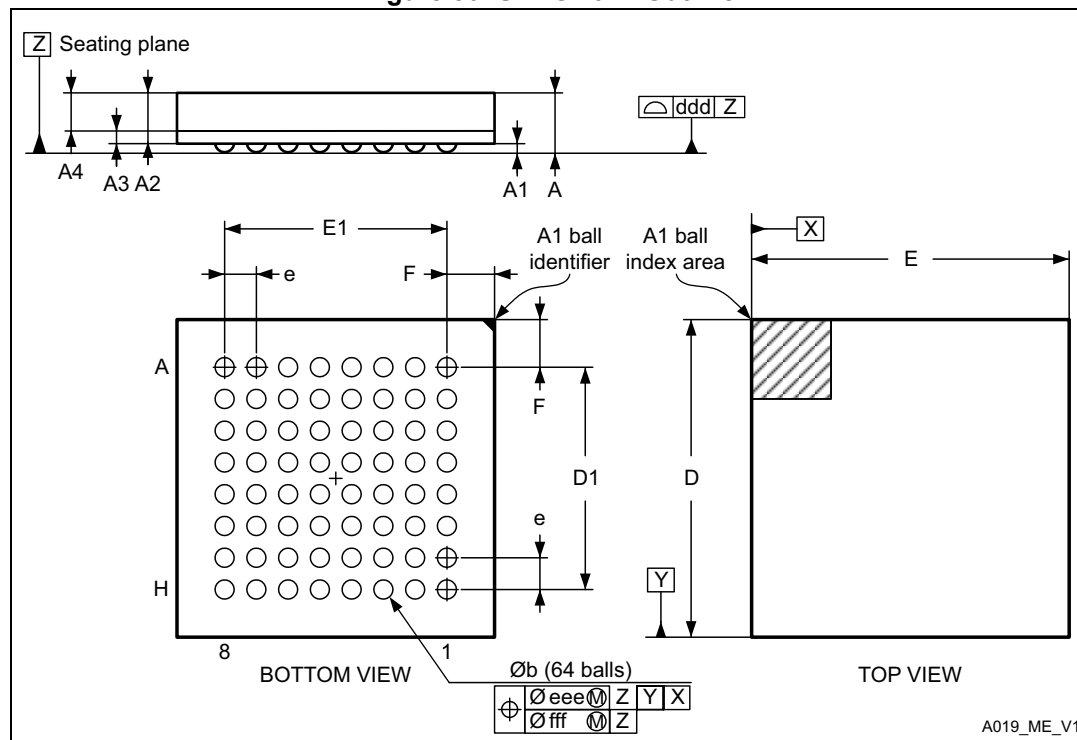
Figure 50. UFBGA64 - Outline
