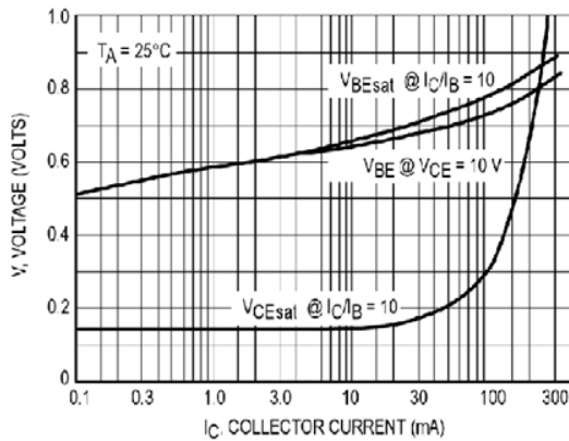
"On" Voltages
