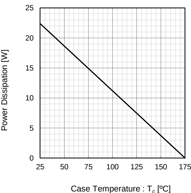
Fig.6 Power Dissipation
