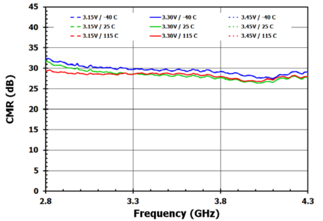
Figure 22. CMR
