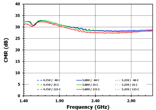
Figure 12. CMR
