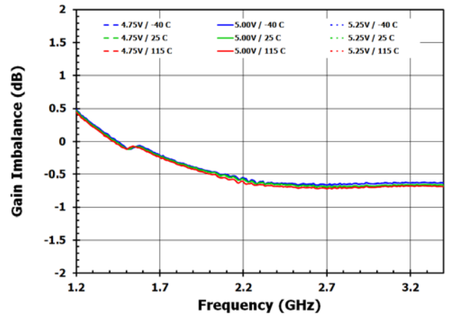
Figure 10. Gain Imbalance
