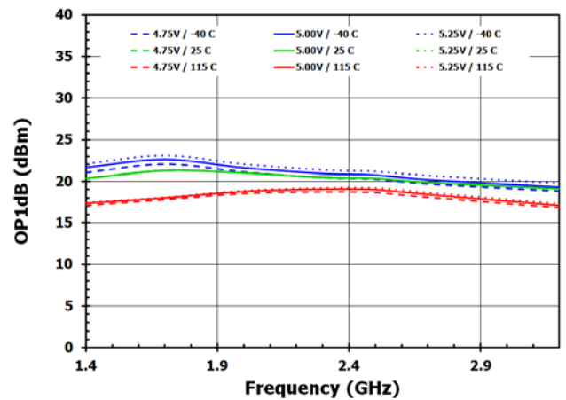
Figure 8. Output P1dB
