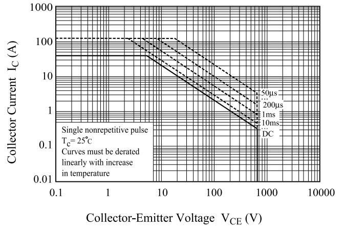
Fig 14. SOA Characteristics
