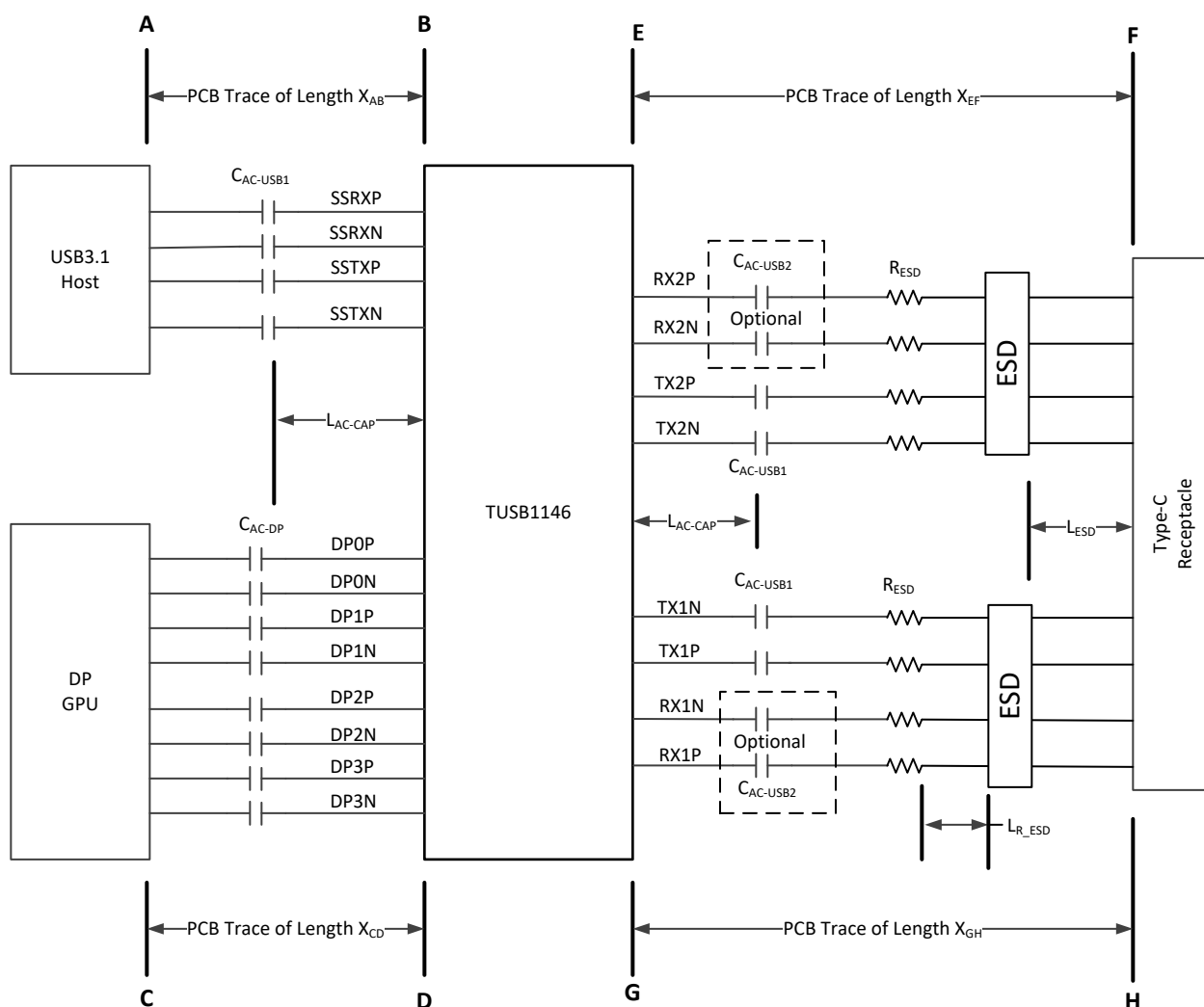
Figure 33. TUSB1146 in a Host Application
