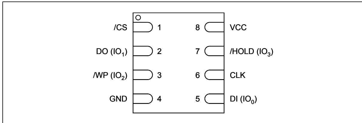
Figure 1b. W25Q16BV Pad Assignments, 8-pad WSON 6x5-mm(Package Code ZP)
