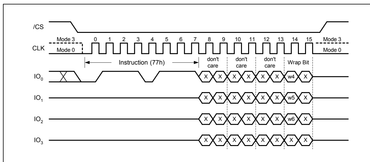
Figure 18. Set Burst with Wrap Instruction (SPI Mode only)
