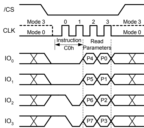
Figure 37. Set Read Parameters Instruction (QPI Mode only)
