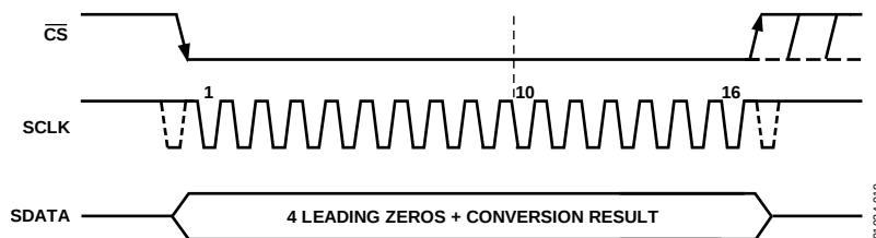
Figure 19. Normal Mode Operation
